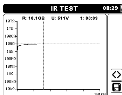
Figure 5.10: Example of Insulation Resistance measurement graph view
