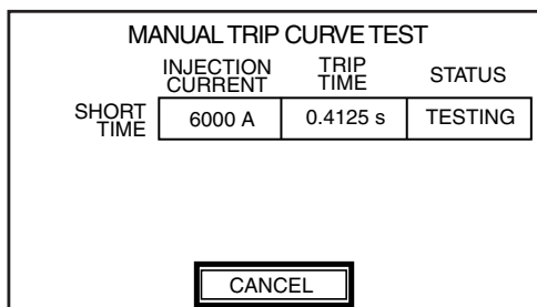
Figure 30 – Manual Trip Curve Test Screen
