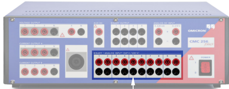
Binary/analog inputs of CMC 256plus
