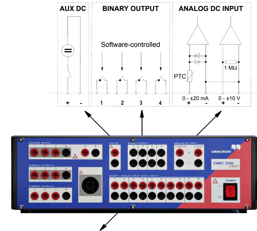
Figure 5-2: Simplified diagrams of analog and binary inputs and outputs
