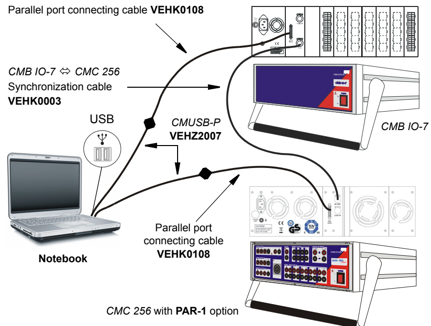
Figure 9-3: Typical test setup with CMB IO-7 , CMC 256 PAR-1 , CMUSB-P and a notebook with USB ports
