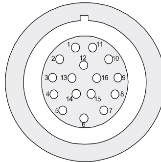
Figure 6-22: Pin assignment of "ext. Interf." (upper 16-pole Lemo socket); view onto the connector from the cable wiring side
