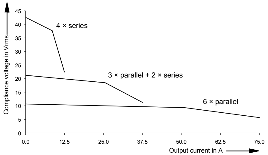
Figure 6-12: Typical compliance voltage (50/60 Hz)
